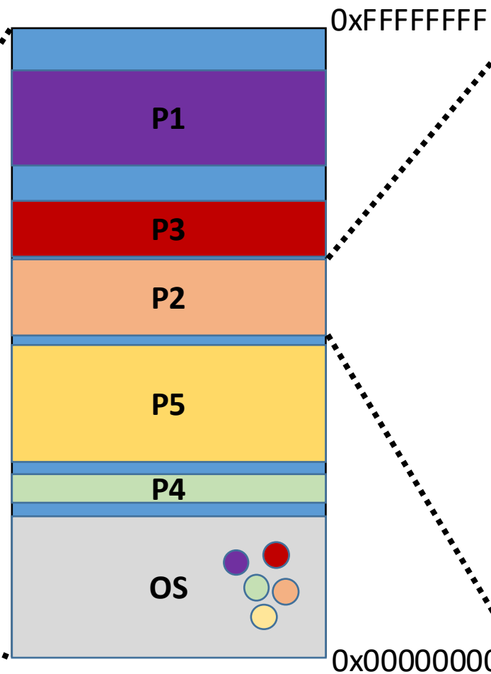
Physical memory
