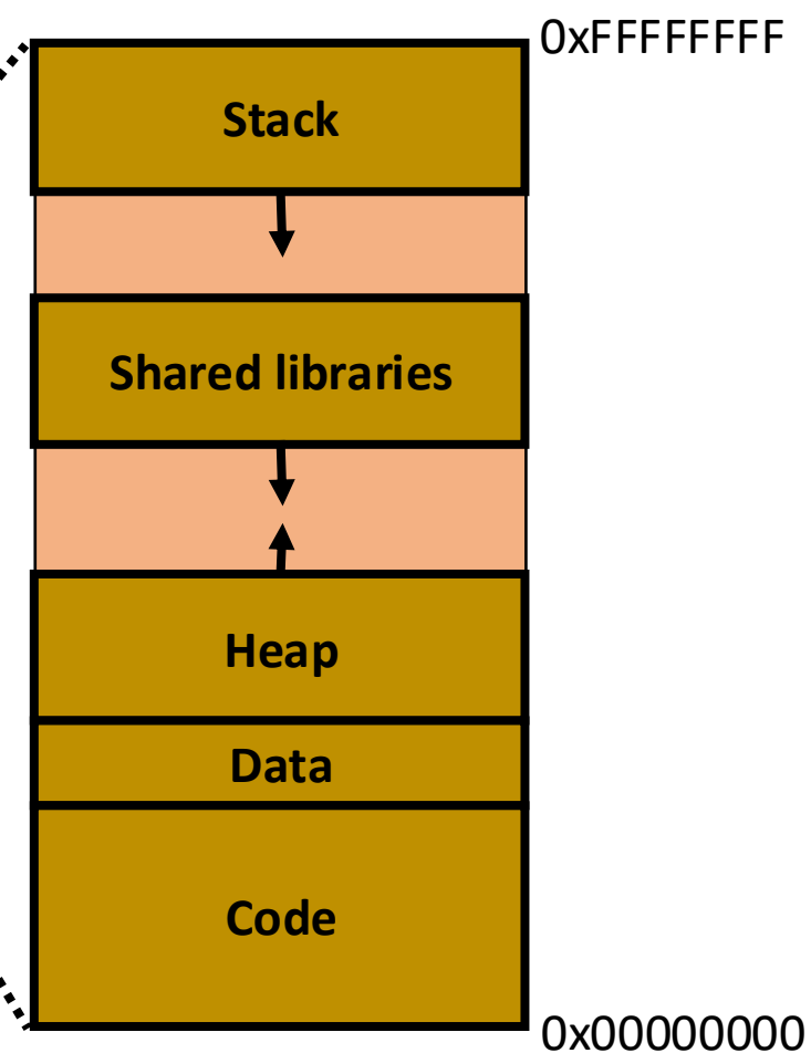
Virtual memory
