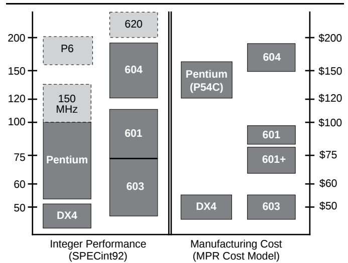
Figure 4. With chips shipping around the end of 1994 (dark gray) and in 1995 (light gray), PowerPC should maintain a significant performance advantage over x86 with comparable factory costs. (Sources: 1994 performance—vendors; 1995 performance—MPR estimates; manufacturing costs—MPR Cost Model)
