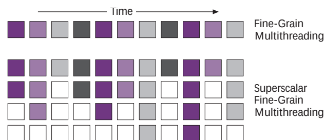
Figure 2. The precursor of SMT, fine-grain multithreading, fills pipeline bubbles by alternating the issue of instructions from several threads. Extending this idea to a superscalar pipeline would fill temporal pipeline bubbles, but, unlike SMT, would not fill execution units in space.
