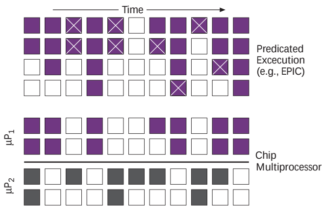
Figure 7. Predicated-execution, such as in Intel and HP's EPIC, tries to fill unused execution slots with speculative operations but often ends up throwing away results (X). Chip multiprocessors, like SMTs, exploit TLP, but they have lower single-thread performance than SMTs for a given amount of resources.
