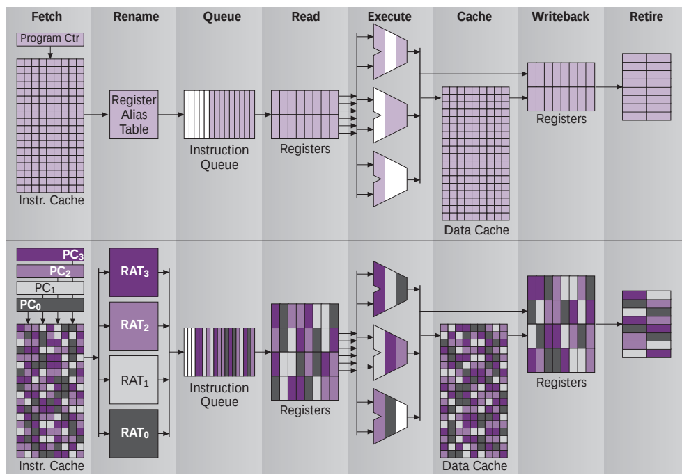
Figure 3. The SMT pipeline (bottom) is similar to a conventional out-of-order superscalar pipeline (top) with the addition of a few thread-specific resources at the front of the pipeline, thread-sensitive BHT and TLBs, and some extra registers.
